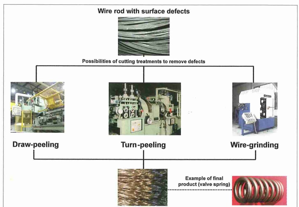
Overview of cutting treatment procedures of wire
