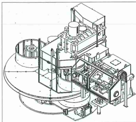
Stand alone draw-peeling machine and Drawing machine with integrated draw-peeling unit
