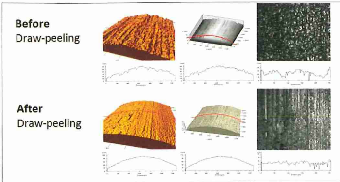
Wire surface after draw-peeling (shaving)
