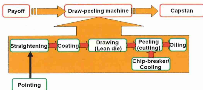
Technological process of draw-peeling
